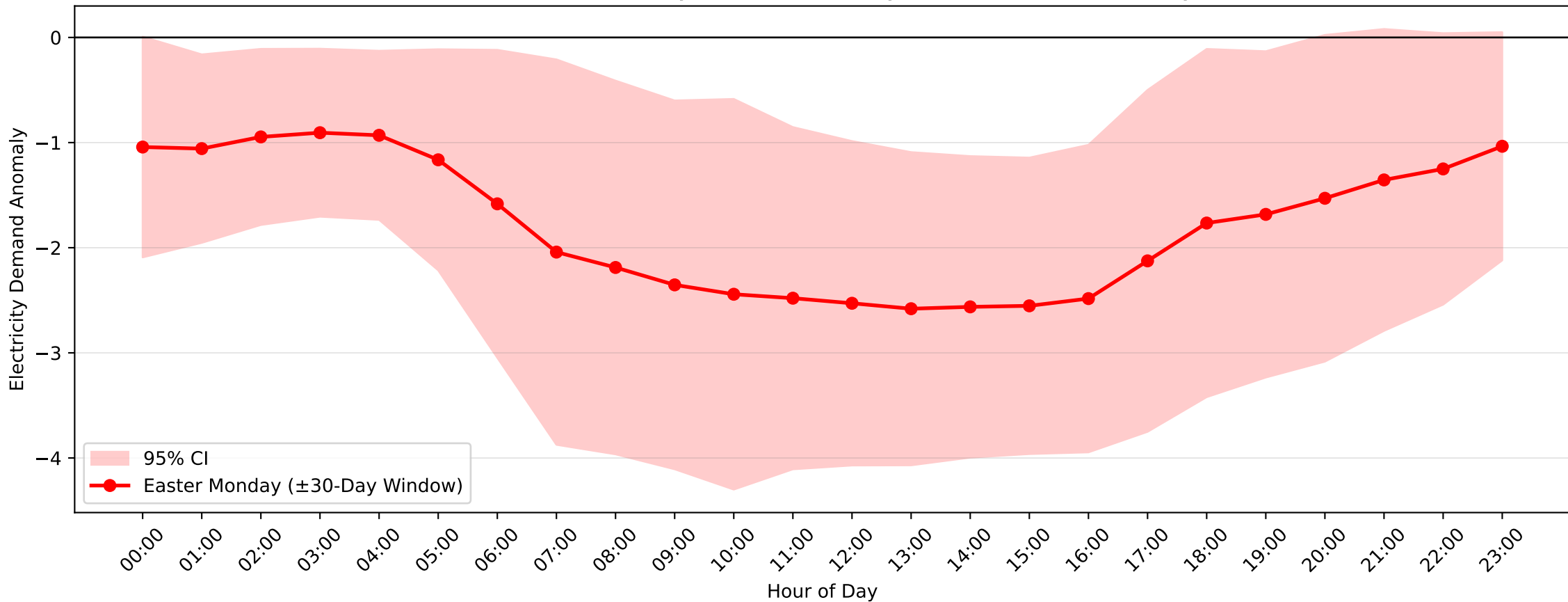
Lidcombe Demand Anomaly: Easter Monday (2004-2017, \pm 30 -Day Window)
